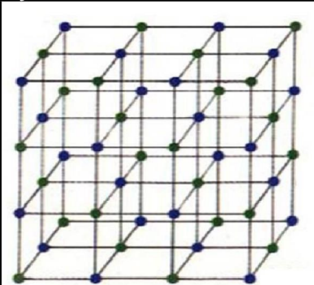
Crystalline three-dimensional-lattice-structure
